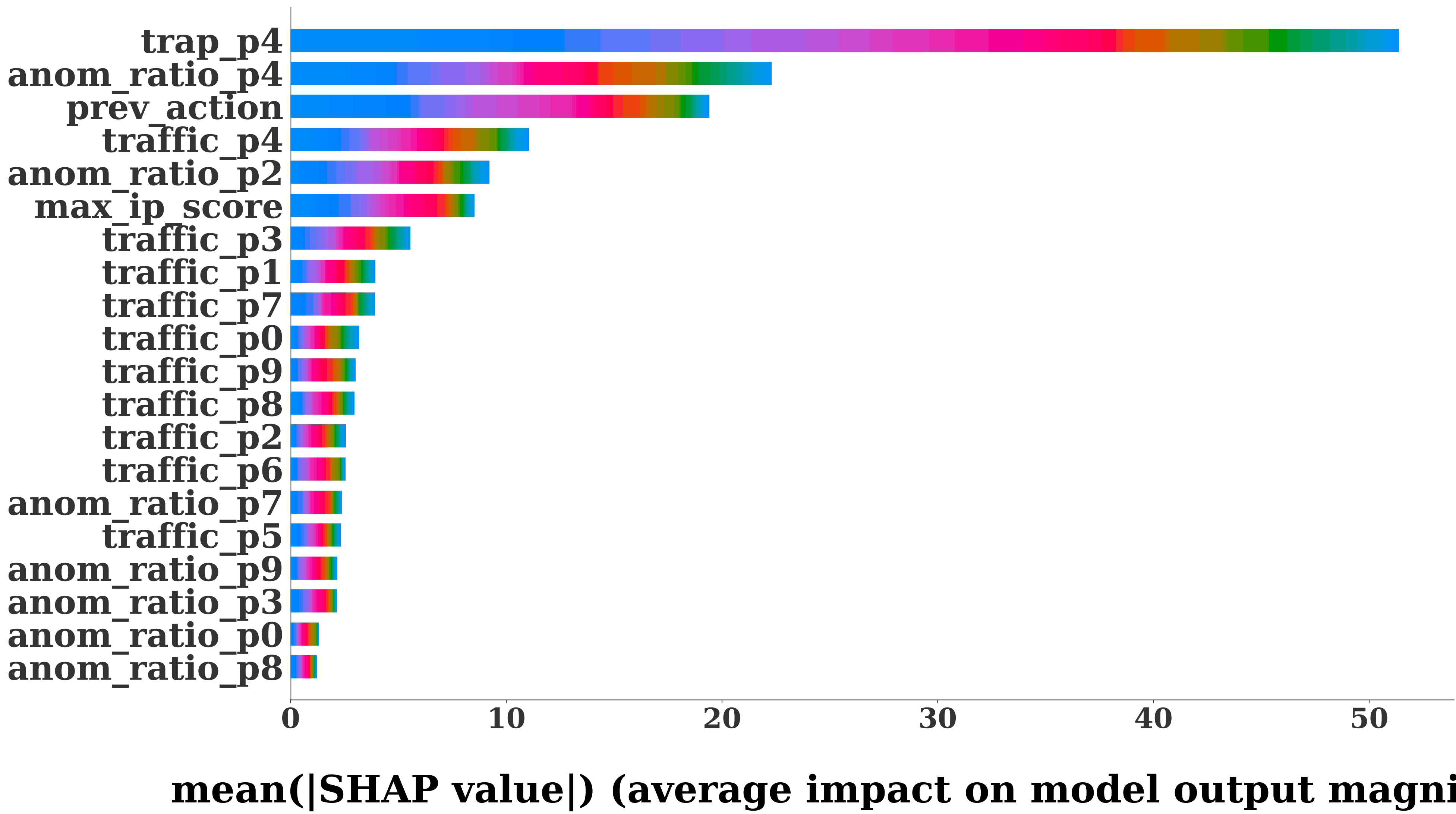
SHAP Action-Feature Interactions: PPO Defender (Seed 2)
